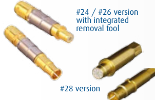
Discrete contacts for D38999 Series III type, Mighty Mouse, SuperNine®, and ARINC 600
