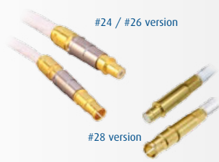
Prewired contacts with Cat 6A aerospace #24, #26, or #28 gage Ethernet cable
